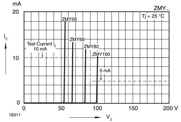
Fig. 8 - Breakdown Characteristics
